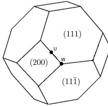
Figure 1: First Brillouin zone of the fcc lattice.
